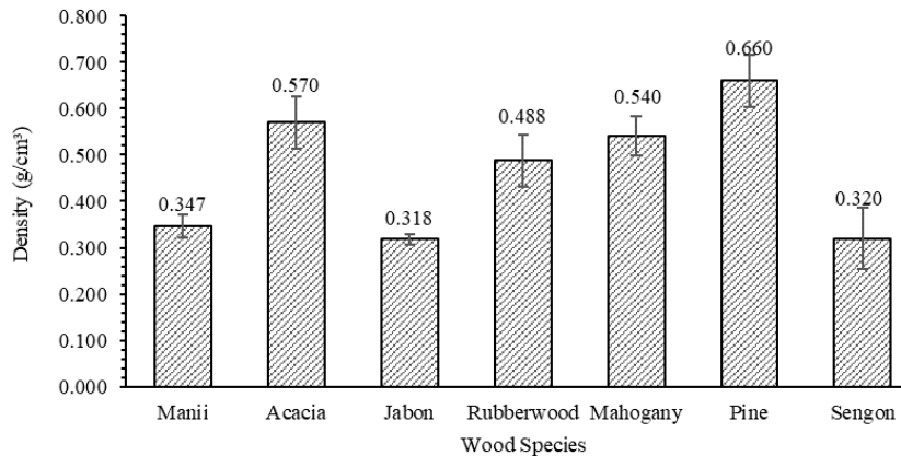
FIGURE 2. The density of seven wood species.
